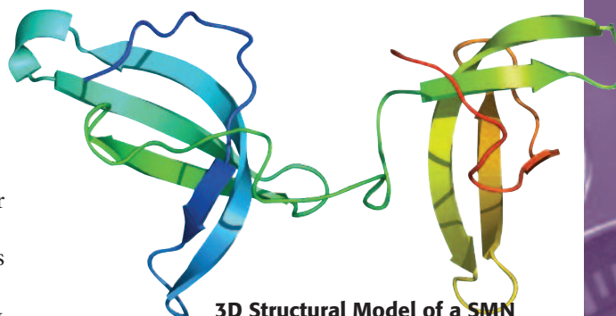
3D Structural Model of a SMN protein fragment, kindly provided by Dr. Allen.
