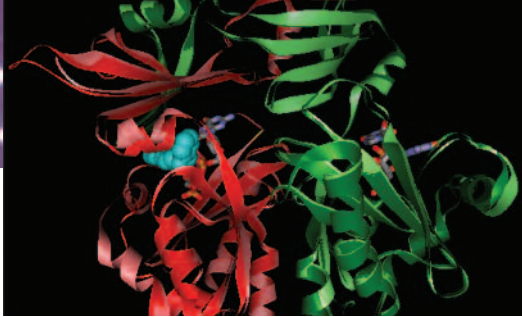
3D Structural Model of a Quinazoline Compound Bound to the Human Enzyme DcpS, from Singh et al 2008.
